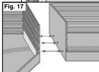
Connector Plates, bolts and wing nuts
