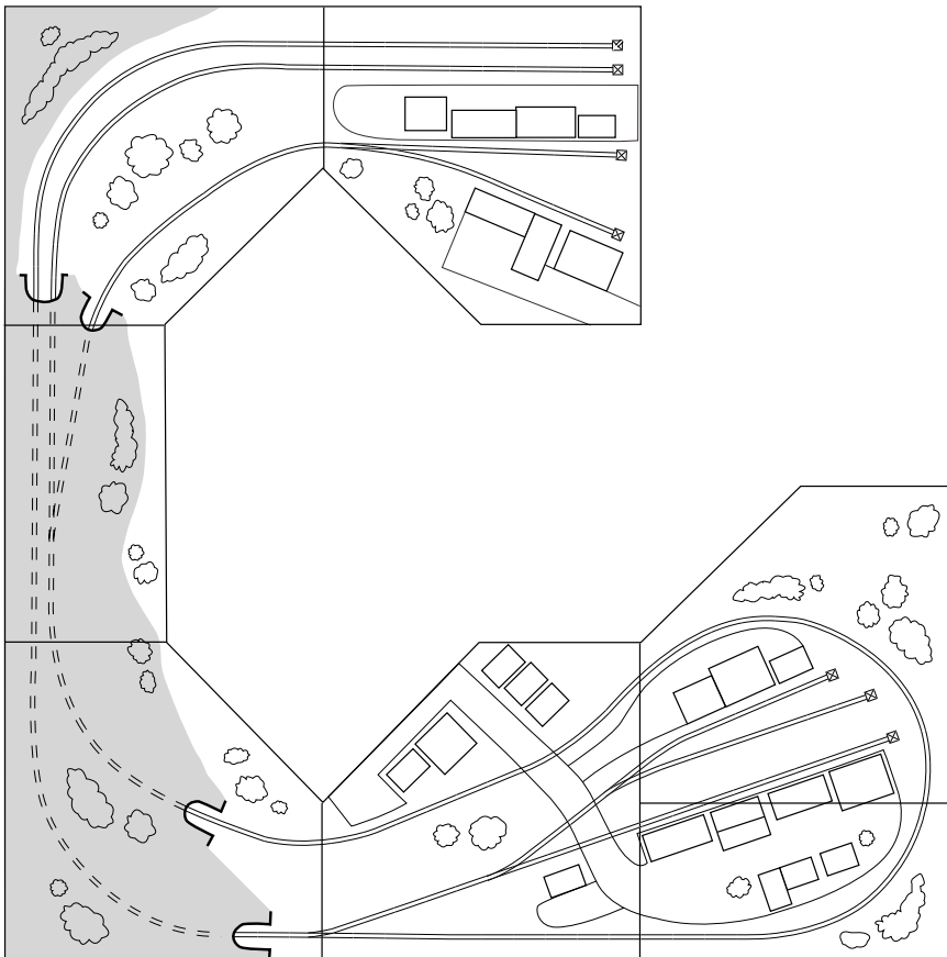
9 x 9-foot Layout 1/2-inch = 1-foot
