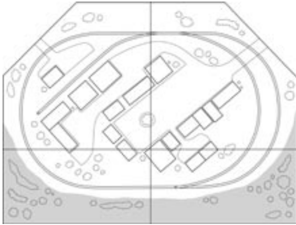
6 x 4 1/2-foot Layout 1/2-inch = 1-foot
