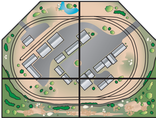
6 x 4 1/2-foot Layout 1/2-inch = 1-foot
